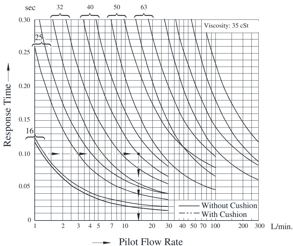
Fig.1 Pilot Flow Rate Vs. Response Time Characteristics Valve size of Logic Valve
