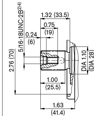
S Splined shaft SAE J744 7/8 in 13 T 16/32 DP 1)
