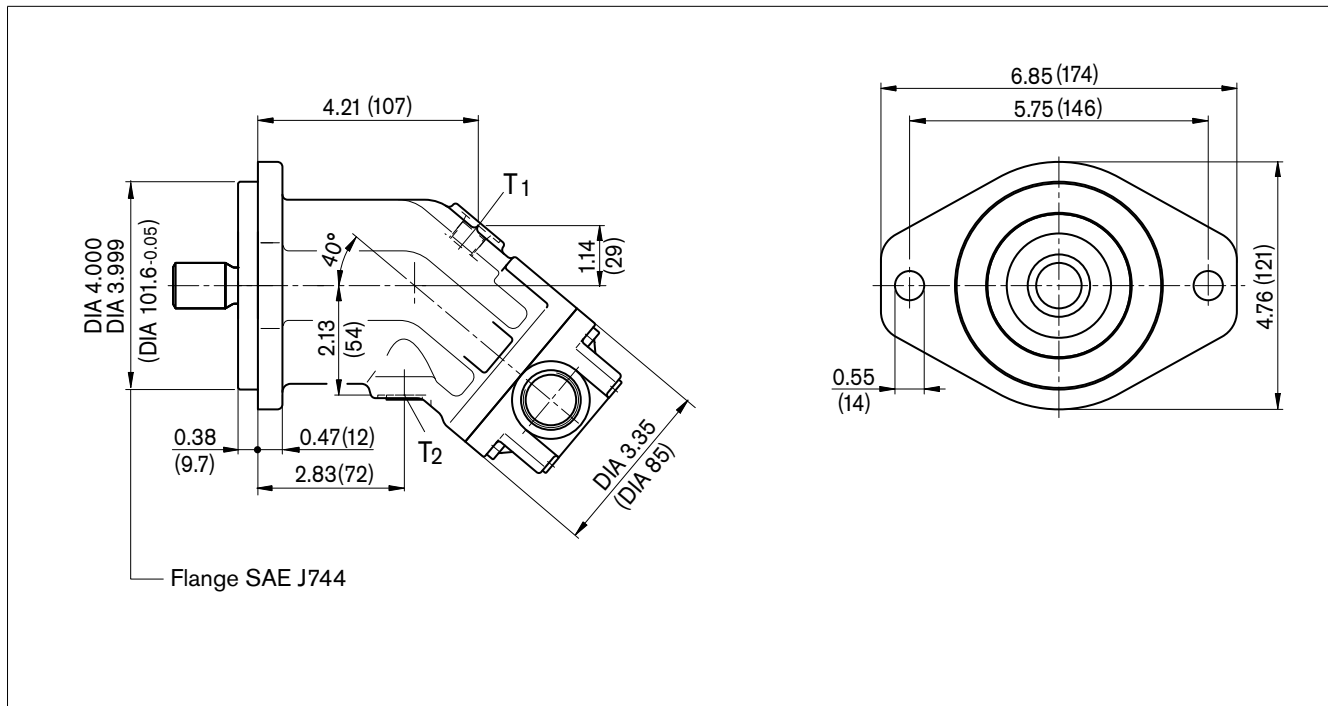
S Splined shaft SAE J744 7/8 in 13 T 16/32 DP 1)
