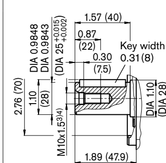
B Parallel keyed shaft, DIN 6885, AS8x7x32 mm
