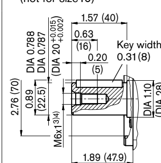
P Parallel keyed shaft DIN 6885, AS8x7x50 (mm) (not for size 16)
